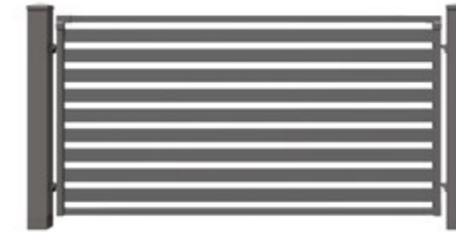
STRAIGHT SEGMENT (TYPE P) Maximum available width: 2500 mm Minimum standard width: 2000 mm
